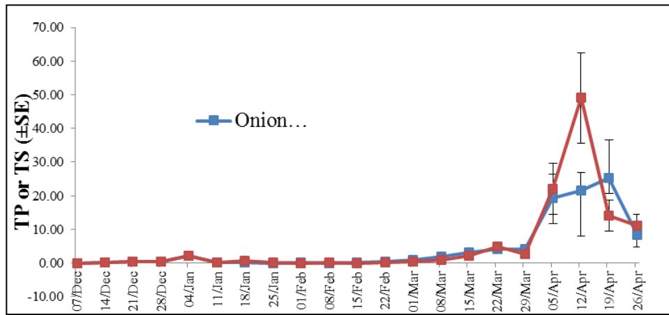
Fig 2: T. tabaci adult on two onion cultivars
