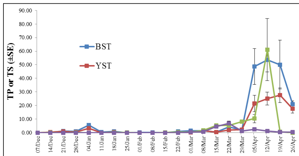
Fig 1: T. tabaci adult counted on sampling methods
